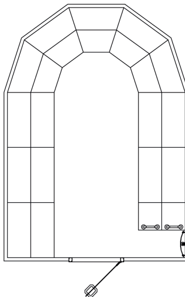
Venus Model 3 Steam Room Size: O.D. 4674mm x 3362mm (I.D. 4540mm x 3242mm) Height: O.D. 2360mm (I.D. 2300mm) 18 - 22 Person seating capacity. 11.4kW - 3 Phase
