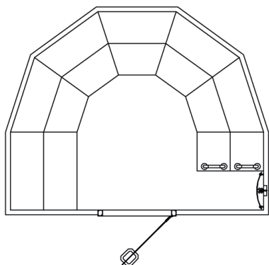
Venus Model 1 Steam Room Size: O.D. 2674mm x 3362mm (I.D. 2540mm x 3242mm) Height: O.D. 2360mm (I.D. 2300mm) 12 - 16 Person seating capacity. 11.4kW - 3 Phase
