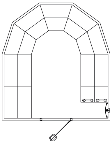
Venus Model 2 Steam Room Size: O.D. 4674mm x 3362mm (I.D. 4540mm x 3242mm) Height: O.D. 2360mm (I.D. 2300mm) 15 - 19 Person seating capacity. 11.4kW - 3 Phase
