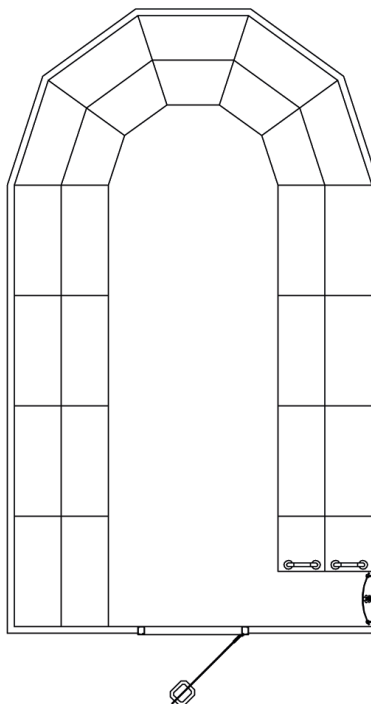
Venus Model 4 Steam Room Size: O.D. 5674mm x 3362mm (I.D. 5540mm x 3242mm) Height: O.D. 2360mm (I.D. 2300mm) 22 - 26 Person seating capacity. 22.8kW - 3 Phase
