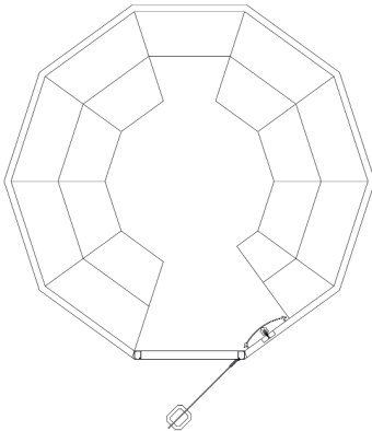
Comfort 1 Steam Room Size: O.D. 3400mm x 3215mm (I.D. 3236mm x 3078mm) Height: O.D. 2360mm (I.D. 2300mm) 12 - 16 Person seating capacity. 11.4kW - 3 Phase
