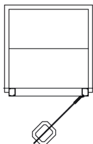
Compact Model 1 Steam Room Size: O.D. 865mm x 850mm (I.D. 750mm x 750mm) Height: O.D. 2190mm (I.D. 2150mm) 1 Person seating capacity. 6.0kW - 1 or 3 Phase
