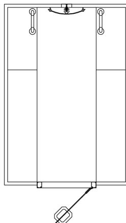
Compact Model 2 Steam Room Size: O.D. 865mm x 1525mm (I.D. 750mm x 1425mm) Height: O.D. 2190mm (I.D. 2150mm) 2 - 3 Person seating capacity. 6.0kW - 1 or 3 Phase
