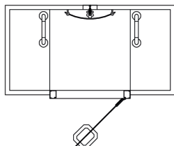
Compact Model 3 Steam Room Size: O.D. 875mm x 1580mm (I.D. 750mm x 1500mm) Height: O.D. 2190mm (I.D. 2150mm) 2 Person seating capacity. 6.0kW - 1 or 3 Phase
