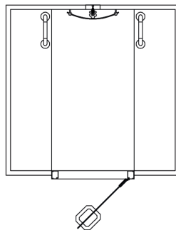
Compact Model 1 Steam Room Size: O.D. 865mm x 850mm (I.D. 750mm x 750mm) Height: O.D. 2190mm (I.D. 2150mm) 1 Person seating capacity. 6.0kW - 1 or 3 Phase
