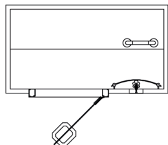
Compact Model 2 Steam Room Size: O.D. 865mm x 1525mm (I.D. 750mm x 1425mm) Height: O.D. 2190mm (I.D. 2150mm) 2 - 3 Person seating capacity. 6.0kW - 1 or 3 Phase
