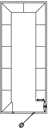
Standard Model 22 Steam Room Size: O.D. 2120mm x 5135mm (I.D. 2000mm x 5000mm) Height: 2260mm 18 - 20 Person seating capacity. 22.8kW - 3 Phase
