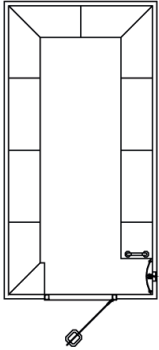
Standard Model 16 Steam Room Size: O.D. 2120mm x 4135mm (I.D. 2000mm x 4000mm) Height: 2260mm 14 - 16 Person seating capacity. 11.4kW - 3 Phase
