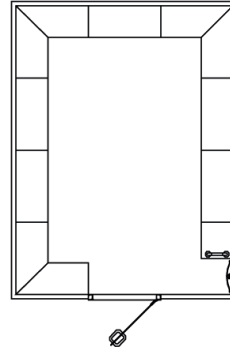
Standard Model 18 Steam Room Size: O.D. 3120mm x 4135mm (I.D. 3000mm x 4000mm) Height: 2360mm 20 - 22 Person seating capacity. 22.8kW - 3 Phase
