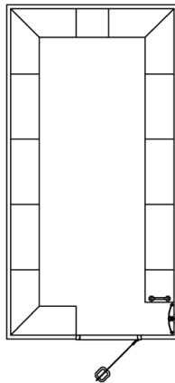
Standard Model 23 Steam Room Size: O.D. 2620mm x 5135mm (I.D. 2500mm x 5000mm) Height: 2310mm 20 - 22 Person seating capacity. 22.8kW - 3 Phase
