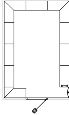
Standard Model 21 Steam Room Size: O.D. 3120mm x 4635mm (I.D. 3000mm x 4500mm) Height: 2360mm 22 - 24 Person seating capacity. 22.8kW - 1 or 3 Phase
