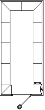
Standard Model 19 Steam Room Size: O.D. 2120mm x 4635mm (I.D. 2000mm x 4500mm) Height: 2360mm 16 - 18 Person seating capacity. 11.4kW - 3 Phase
