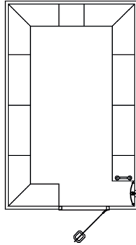
Standard Model 17 Steam Room Size: O.D. 2620mm x 4135mm (I.D. 2500mm x 4000mm) Height: 2310mm 18 - 20 Person seating capacity. 11.4kW - 1 or 3 Phase
