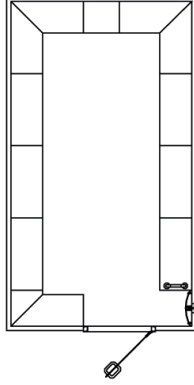
Standard Model 20 Steam Room Size: O.D. 2620mm x 4635mm (I.D. 2500mm x 4500mm) Height: 2310mm 18 - 20 Person seating capacity. 11.4kW - 3 Phase
