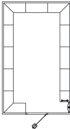
Standard Model 24 Steam Room Size: O.D. 3120mm x 5135mm (I.D. 3000mm x 5000mm) Height: 2360mm 24 - 26 Person seating capacity. 22.8kW - 3 Phase
