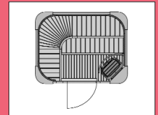
Model: SD2015 Size: 1940 x 1500 Seats: 3-4 Stove: 6.0kW
