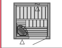
Model: S1010 Size: 1000 x 1000 Seats: 2-3 Stove: 2.3kW
