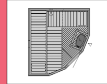
Model: S2522M Size: 2380 x 2195 Seats: 6-7 Stove: 8.0kW
