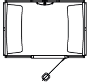
Sedna Model 2 Steam Room Size: O.D. 2330mm x 1626mm Height: O.D. 2265mm 4 Person seating capacity. 6.0kW - 1 or 3 Phase
