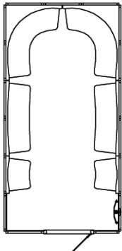
Sedna Model 12 Steam Room Size: O.D. 2330mm x 4580mm Height: O.D. 2265mm 12 Person seating capacity. 11.4kW - 1 or 3 Phase
