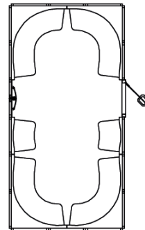
Sedna Model 15 Steam Room Size: O.D. 2330mm x 4580mm Height: O.D. 2265mm 14 Person seating capacity. 11.4kW - 1 or 3 Phase
