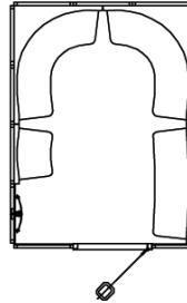
Sedna Model 6 Steam Room Size: O.D. 2330mm x 3103mm Height: O.D. 2265mm 9 Person seating capacity. 11.4kW - 1 or 3 Phase
