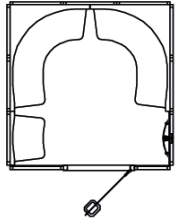
Sedna Model 4 Steam Room Size: O.D. 2330mm x 2353mm Height: O.D. 2265mm 7 Person seating capacity. 6.0kW - 1 or 3 Phase
