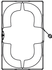
Sedna Model 10 Steam Room Size: O.D. 2330mm x 3830mm Height: O.D. 2265mm 12 Person seating capacity. 11.4kW - 1 or 3 Phase
