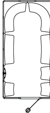
Sedna Model 14 Steam Room Size: O.D. 2330mm x 4603mm Height: O.D. 2265mm 13 Person seating capacity. 11.4kW - 1 or 3 Phase
