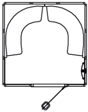
Sedna Model 3 Steam Room Size: O.D. 2330mm x 2330mm Height: O.D. 2265mm 6 Person seating capacity. 6.0kW - 1 or 3 Phase
