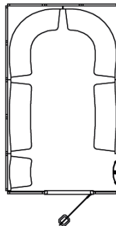
Sedna Model 9 Steam Room Size: O.D. 2330mm x 3853mm Height: O.D. 2265mm 11 Person seating capacity. 11.4kW - 1 or 3 Phase
