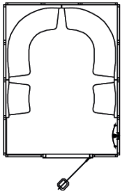
Sedna Model 5 Steam Room Size: O.D. 2330mm x 3080mm Height: O.D. 2265mm 8 Person seating capacity. 11.4kW - 1 or 3 Phase
