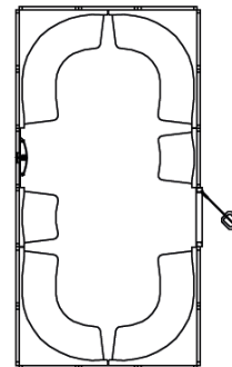
Sedna Model 16 Steam Room Size: O.D. 2330mm x 4580mm Height: O.D. 2265mm 14 Person seating capacity. 11.4kW - 1 or 3 Phase
