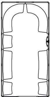
Sedna Model 13 Steam Room Size: O.D. 2330mm x 4603mm Height: O.D. 2265mm 13 Person seating capacity. 11.4kW - 1 or 3 Phase
